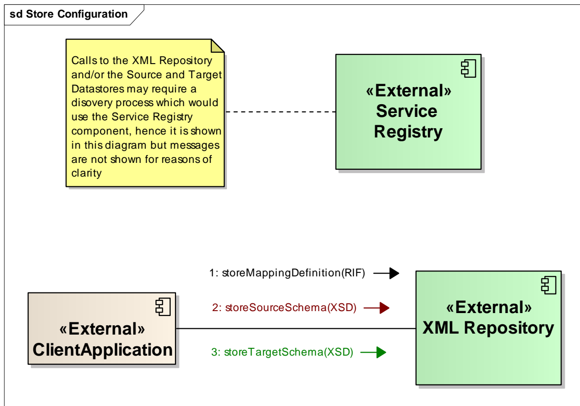
Figure 8 Store Configuration Communication Diagram
